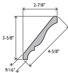
EC47 CROWN 9/16 X 4-5/8
