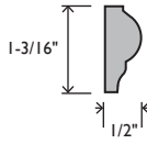
ECI39 PANEL 1/2 X 1-3/16 PRIMED PINE #041392
