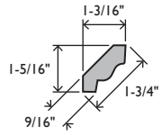
EC60 CROWN 9/16 X 1-3/4 SOLID PINE #00060
