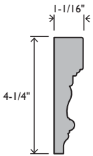
EC414 CASING 1-1/16 X 4-1/4 PRIMED PINE #044142
