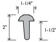
EC1305 ASTRAGAL 1-1/4 X 2
