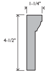
EC190 BRICK MOULD 1-1/4 X 4-1/2
