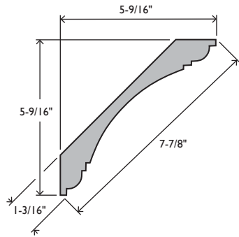
EC778 CROWN 1-3/16 X 7-7/8 PRIMED MDF 28mm #0497785
