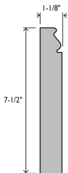
EC26 PLINTH 1-1/8 X 3-1/2 X 7-1/2
