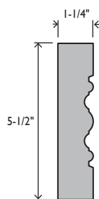
EC25 ROSETTE 1-1/4 X 5-1/2 X 5-1/2
