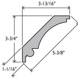
EC39 CROWN 1-1/16 X 5-3/8
