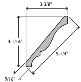
EC45 CROWN 9/16 X 5-1/4
