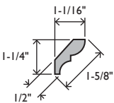
EC75 CROWN 1/2 X 1-5/8 SOLID PINE #00075 PRIMED PINE #040752
