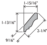
EC54 CROWN 9/16 X 2-1/4 SOLID PINE #00054 PRIMED PINE #040542
