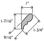
EC74 CROWN 9/16 X 1-3/4 SOLID PINE #00074 PRIMED PINE #040742
