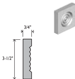
EC30 ROSETTE 3/4 X 3-1/2 X 3-1/2
