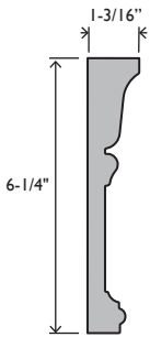
EC625 CASING 1-3/16 X 6-1/4 PRIMED MDF 30mm #046254
