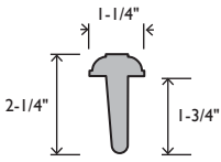
EC1300 ASTRAGAL 1-1/4 X 2-1/4
