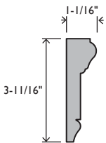
EC460 CASING 1-1/16 X 3-11/16 PRIMED PINE #044602 PRIMED MDF 25mm #044605
