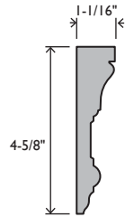
EC466 CASING 1-1/16 X 4-5/8 PRIMED PINE #044662
