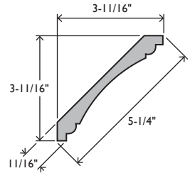
EC50 CROWN 1 1/16 X 5-1/4
