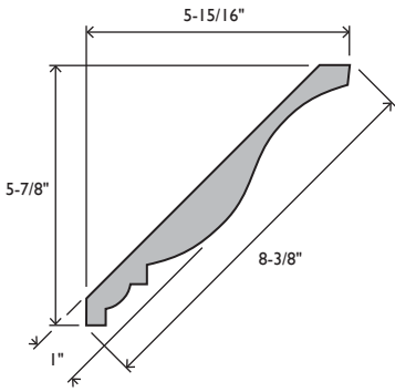
EC838 CROWN 1 X 8-3/8 PRIMED MDF 25mm #0498385
