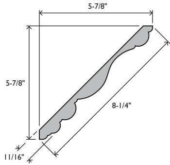
EC814 CROWN 11/16 X 8-1/4 PRIMED MDF 18mm #0498145
