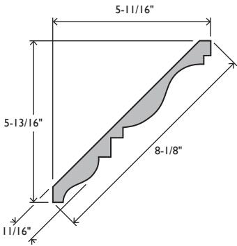
EC818 CROWN 11/16 X 8-1/8 PRIMED MDF 18mm #0498185
