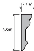
EC446 CASING 1-1/16 X 3-5/8 PRIMED PINE #044462
