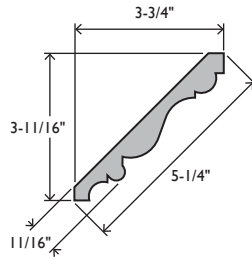
EC36A CROWN 1 1/16 X 5-1/4
