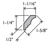
EC68 CROWN 1/2 X 1-5/8 PRIMED PINE #040682
