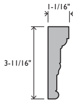
EC470 CASING 1-1/16 X 3-11/16 PRIMED PINE #044702 PRIMED MDF 25mm #044705
