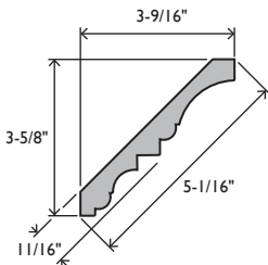
EC37 CROWN 1 1/16 X 5-1/16
