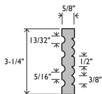
EC14 CASING 5/8 X 3-1/4 PRIMED PINE #040142
