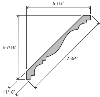
EC734 CROWN 11/16 X 7-3/4 PRIMED MDF 18mm #0497345
