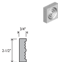
EC29 ROSETTE 3/4 X 2-1/2 X 2-1/2
