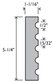
EC514 CASING 1-1/16 X 5-1/4 FINGERJOINT PINE #10514
