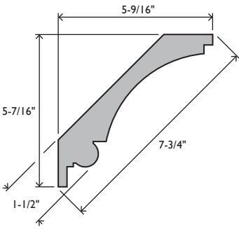
EC24 CROWN 1-1/2 X 7-3/4 PRIMED PINE #040242
