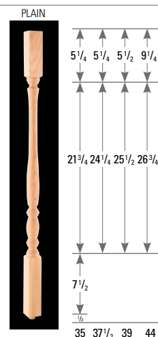
2105 Crown System 1 3/4"
