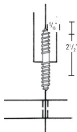
3076-20/ 3076-50 Dowel Screws Fully-threaded dowel screws for attaching balusters to treads. Available in packs of 20 or 50.
