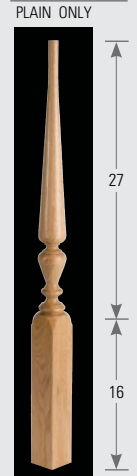
8512 (43") Rake Newel
