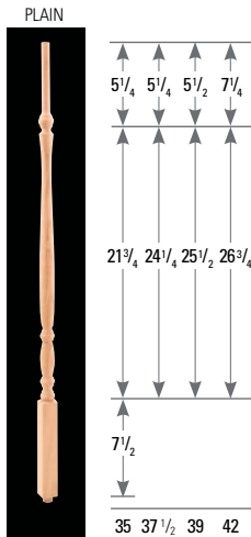
2013 Crown System* 1 1/4"
