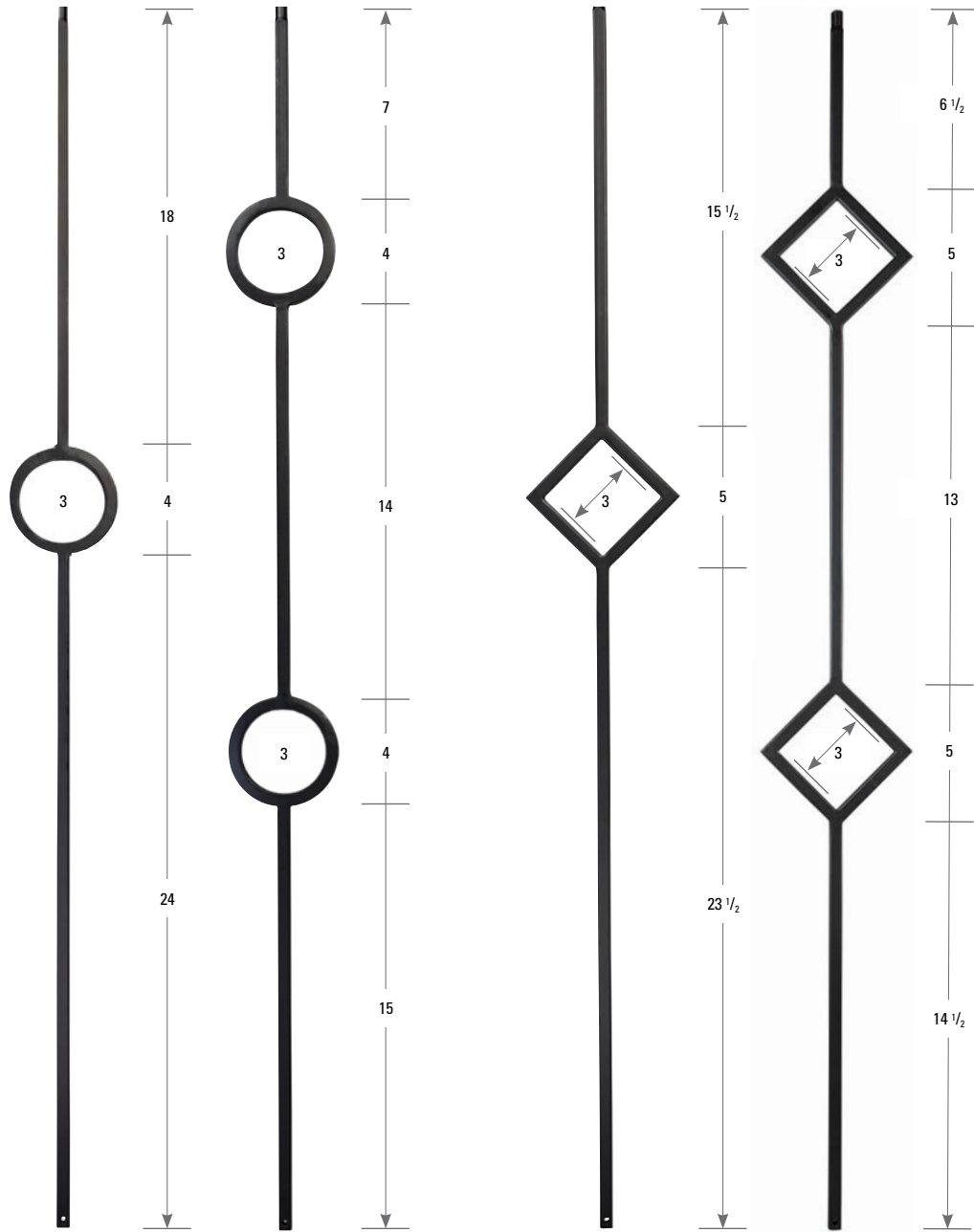
3401 (Hollow) 12mm
