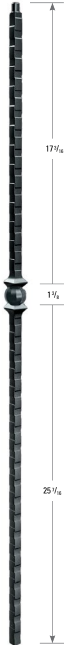
1061 (Solid) 14mm
