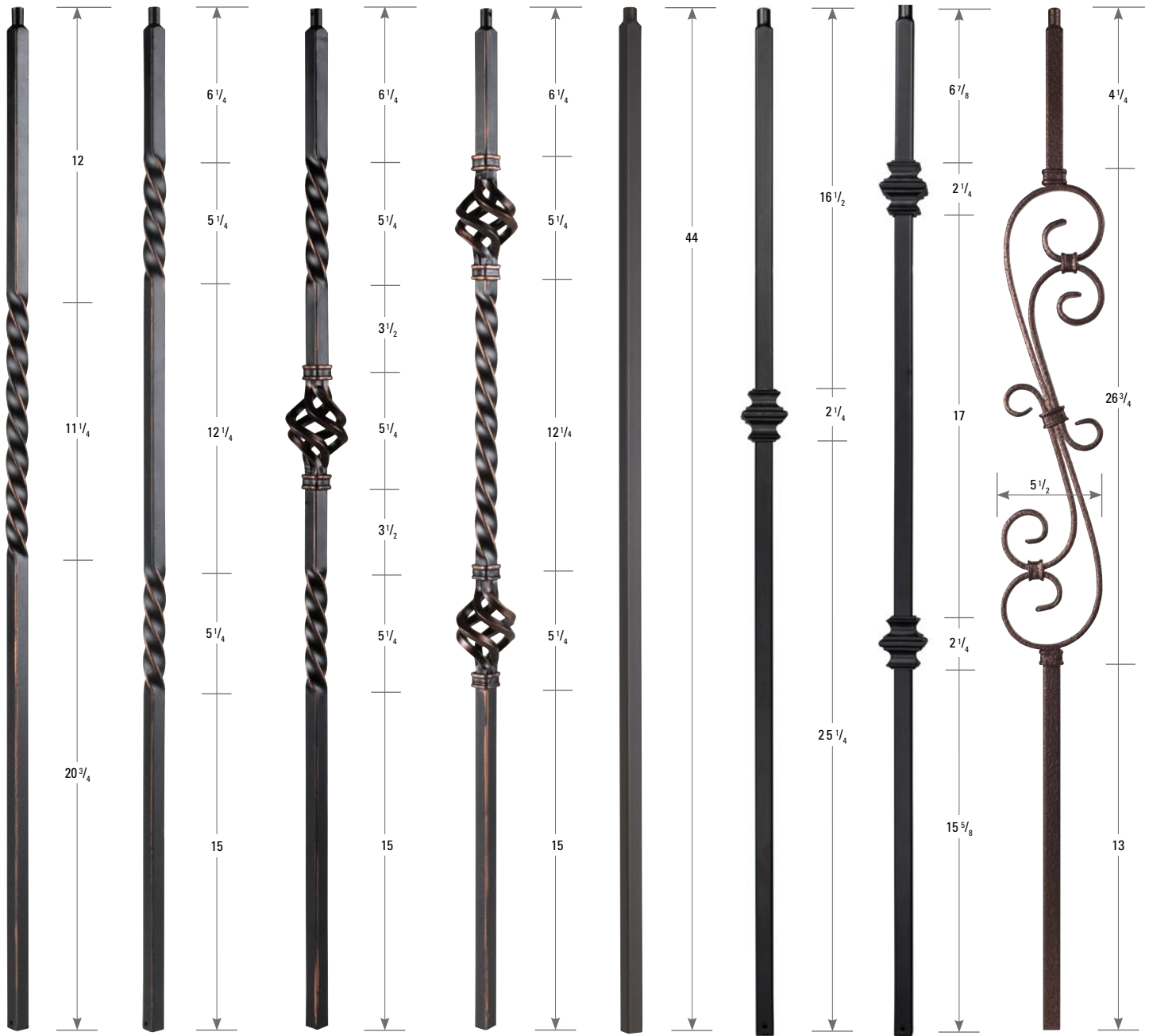
2101 (Hollow) 19mm
