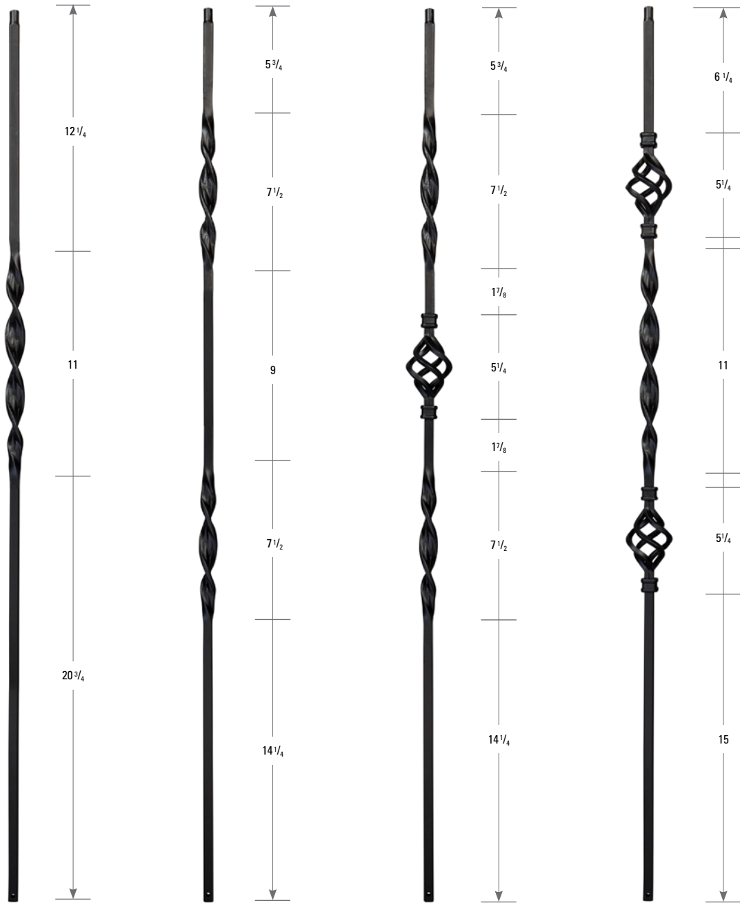
3301 (Hollow) 12mm
