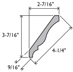
EC48 CROWN 9/16 X 4-1/4 SKU: MLD0048FJ REF: 8012
