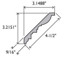
EC7022 CROWN 9/16 X 4-1/2 SKU: MLD0022FJC REF: CR22
