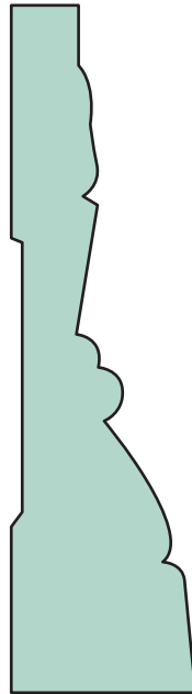
WM 314 C,P 7/8 X 3-1/4 NEW ORLEANS
