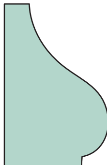
WM 166 L 1-1/8 X 1-3/4
