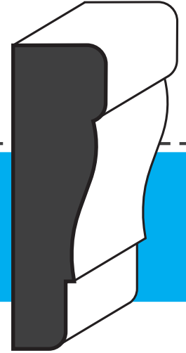
EC 356 GEARScan 2-1/4" 000356
