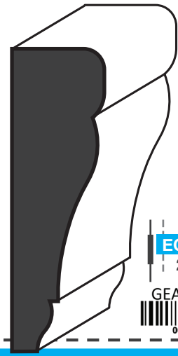
EC 366 2-1/4"
