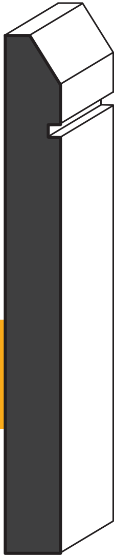
EC 705 5-1/4"
