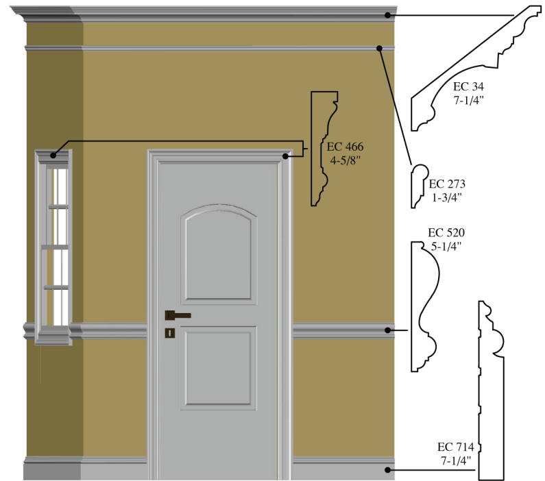
12 ft. Ceiling with an 8 ft. Door
